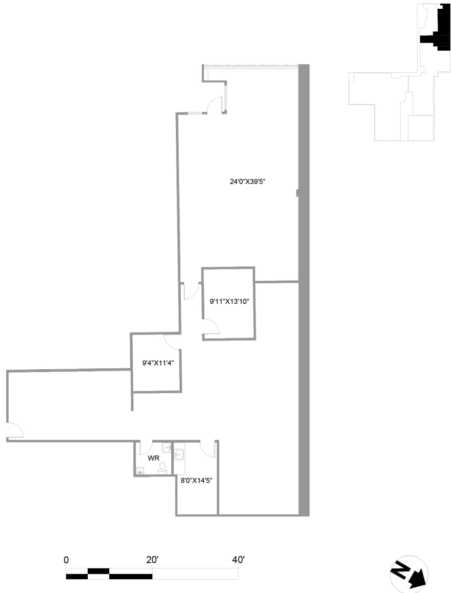
KEY PLAN
